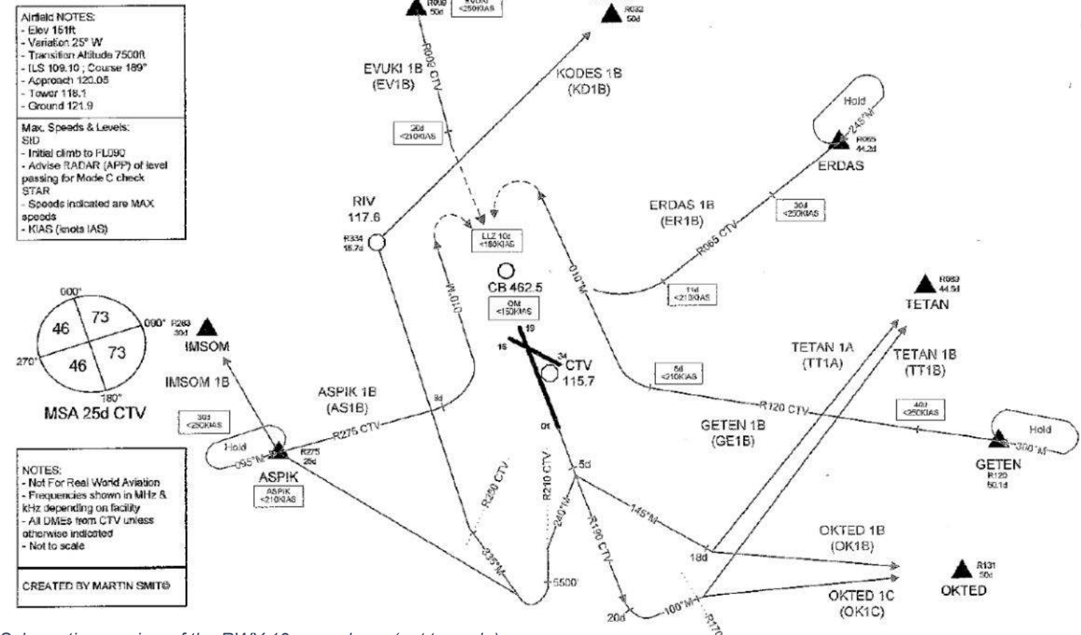
Schematic overview of the RWY 19 procedures (not to scale).
