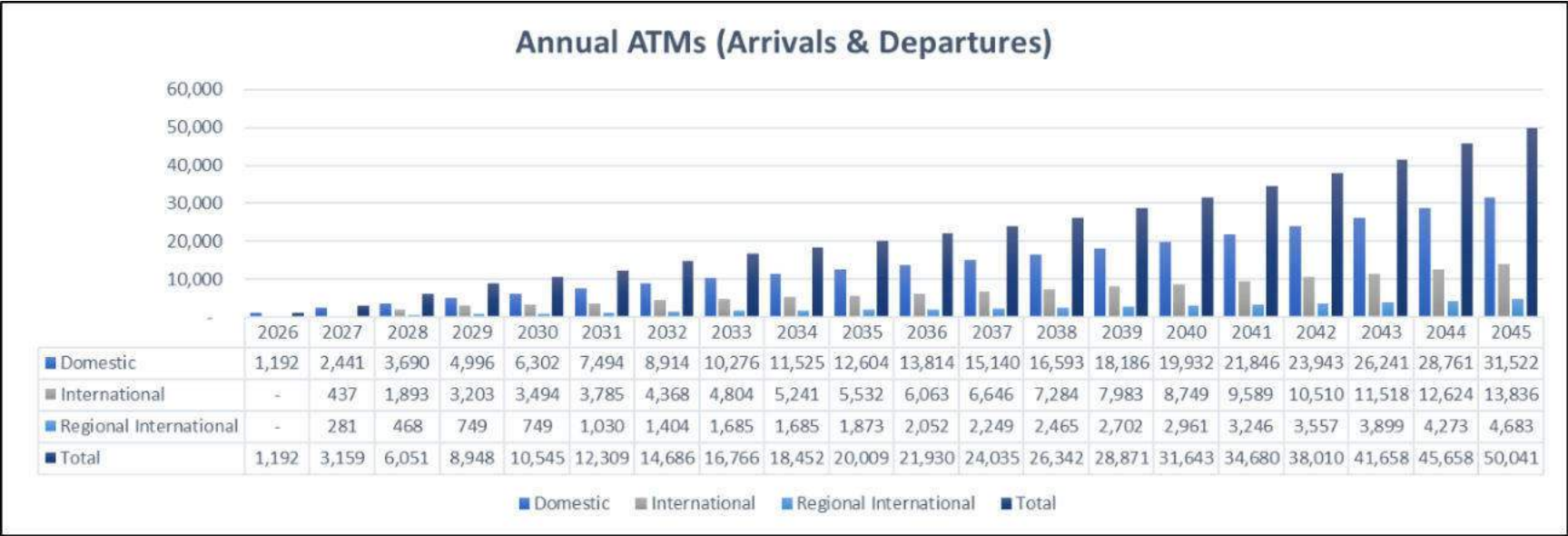
Forecast scheduled annual air traffic movements, from file: 2022-08-19 Traffic Forecast (Consultants)
