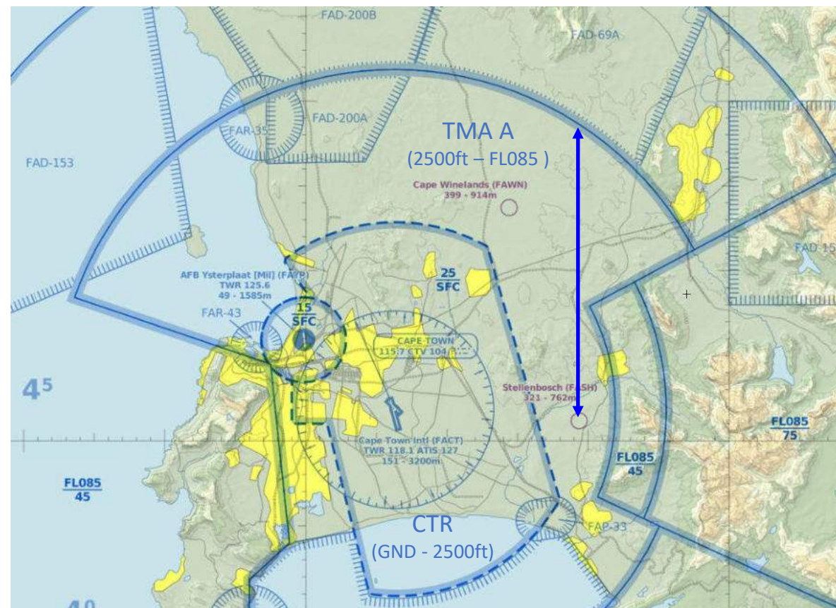
VFR aeronautical chart
