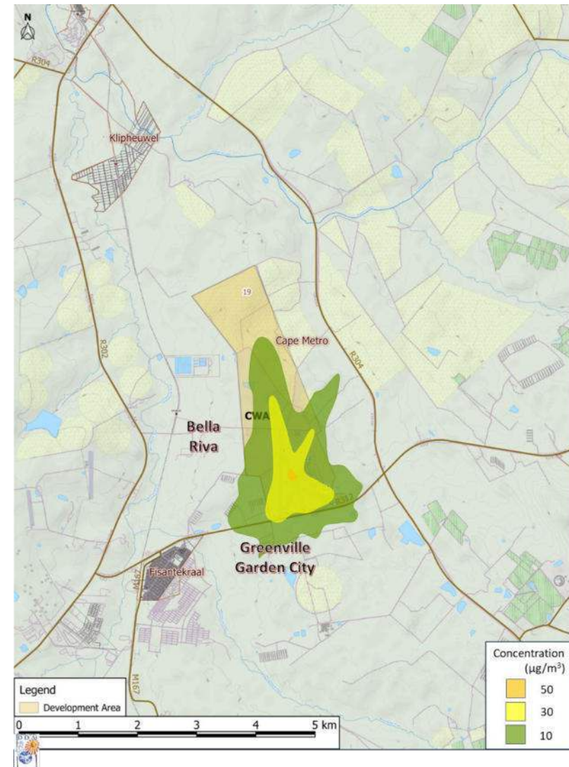
Figure 5-6. Scenario 1: SO 2 1-hr Maximum Concentrations (Guideline value: 350 µg/m³)
