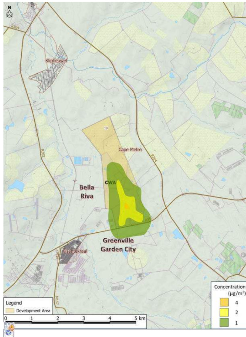
Figure 5-5. Scenario 1: NO 2 Maximum Annual Concentrations (Guideline: 40 µg/m³)
