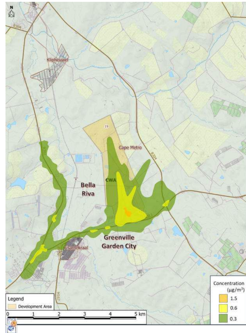
Figure 5-8. Scenario 1: \text{PM}_{10} 24-hr Maximum Concentrations (Guideline 120 \mu\text{g}/\text{m}^3 )
