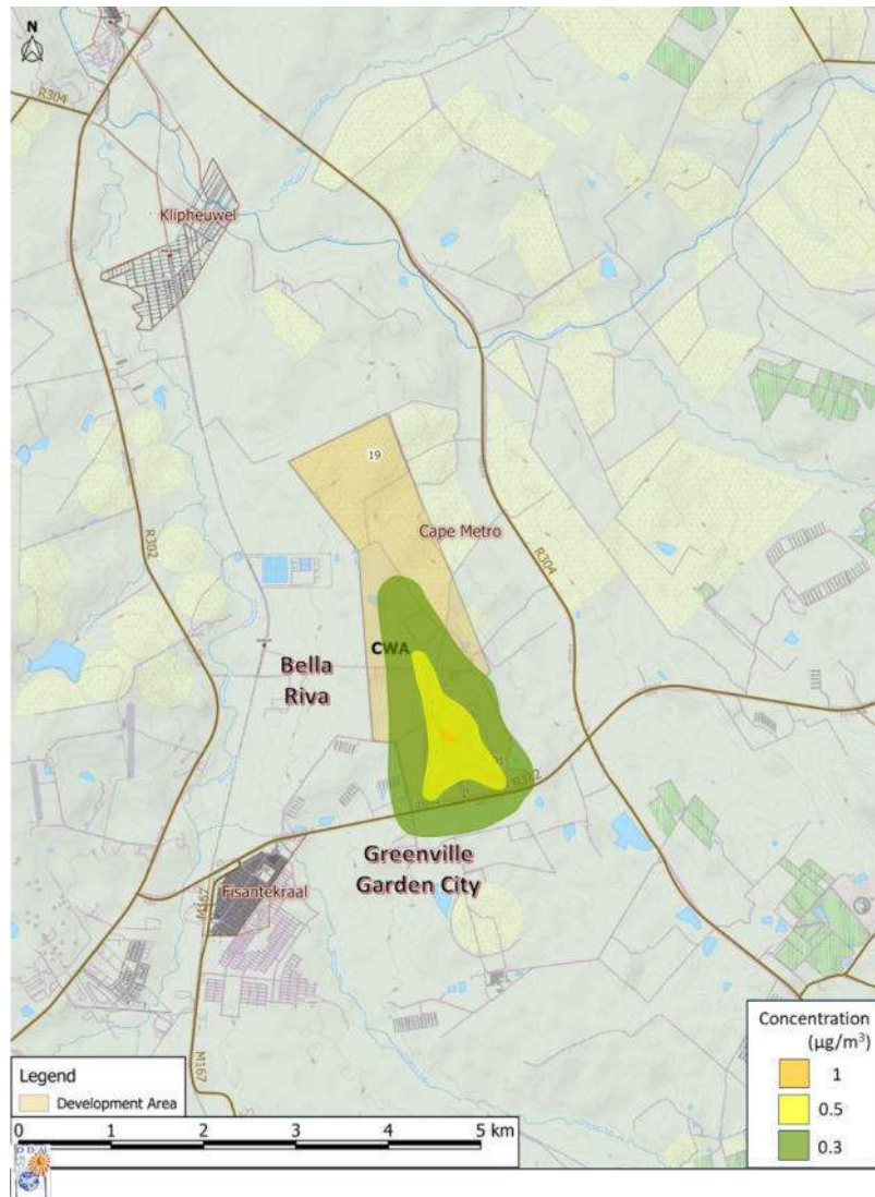
Figure 5-7. Scenario 1: \text{SO}_2 Maximum Annual Concentrations (Guideline: 50 \mu\text{g}/\text{m}^3 )
